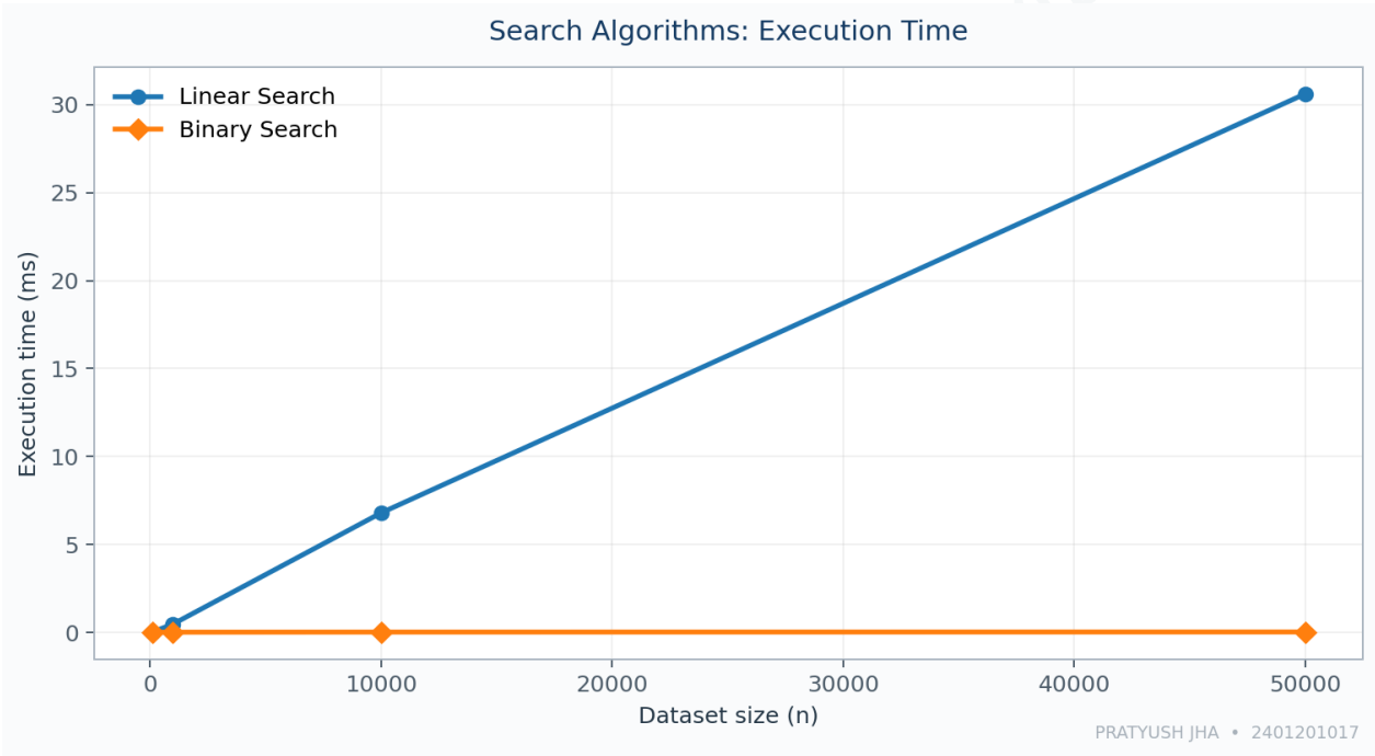
Figure 1. Dataset size vs execution time for Linear and Binary Search
