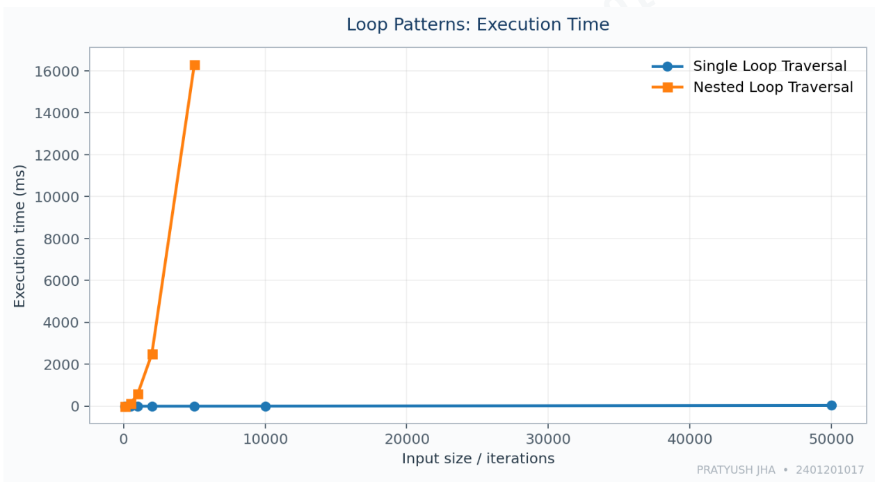
Figure 3. Execution time comparison of Single Loop and Nested Loop
