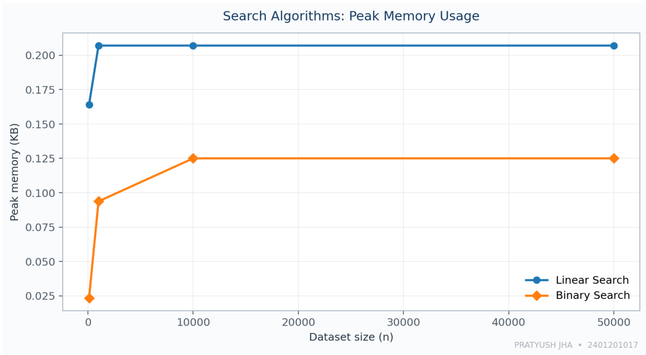
Figure 2. Peak memory usage for Linear and Binary Search
