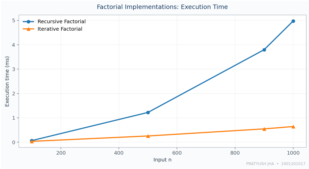
Figure 4. Execution time comparison of Recursive and Iterative Factorial
